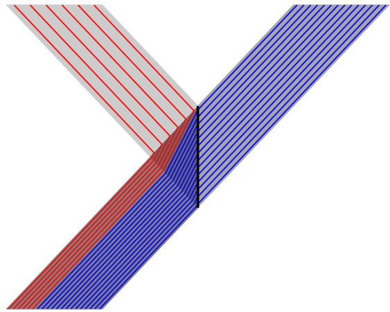
FIG. 7: A wave packet passing through a beam splitter, in the Many Bohmian Worlds picture. In this example, there is a chance of 70% to cross the beam splitter. The gray areas represent the incident, transmitted and reflected wave functions. Blue trajectories represent particles which get through the beam splitter, while red trajectories represent reflected particles.
