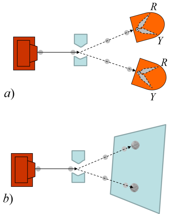
FIG. 3: a). The Stern-Gerlach experiment with pointer displays. R refers to READY position and Y to YES position of the pointer which signifies detection of the atom. The superposition of the wave packets of the atom creates an entangled superposition of the two pointers which collapses almost to a product state due to the first GRW hit. b). The Stern-Gerlach experiment with a screen display. The superposition of the wave packets of the atom creates an entangled superposition of the internal states of a macroscopic number of atoms on the screen. This superposition does not collapse due to the GRW hits, so the definite result of the measurement will take place at a much later stage.
